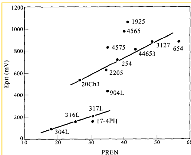
Fig. 6. Plots of PREN of different steels vs pitting potential in seawater
